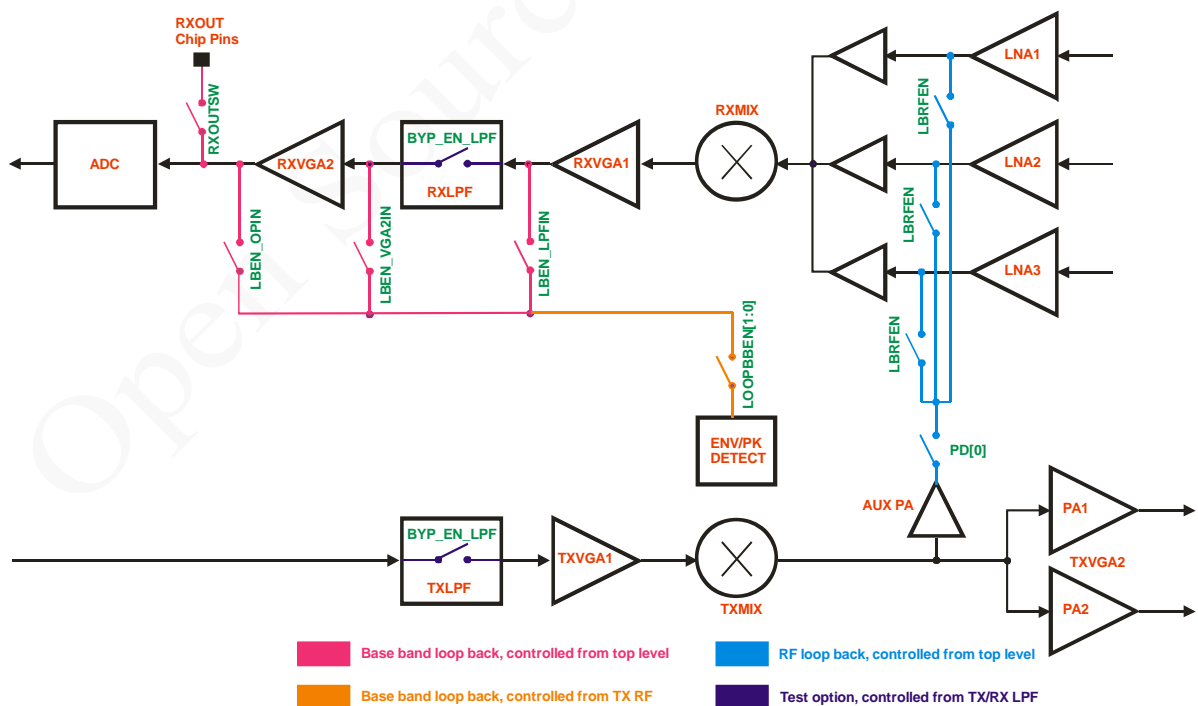
Figure 3.1: Loop back and test options
