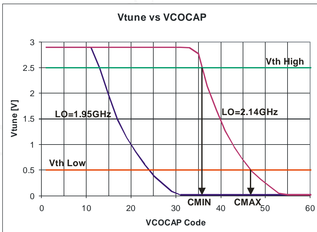
Figure 3.3: VCO capacitance selection
